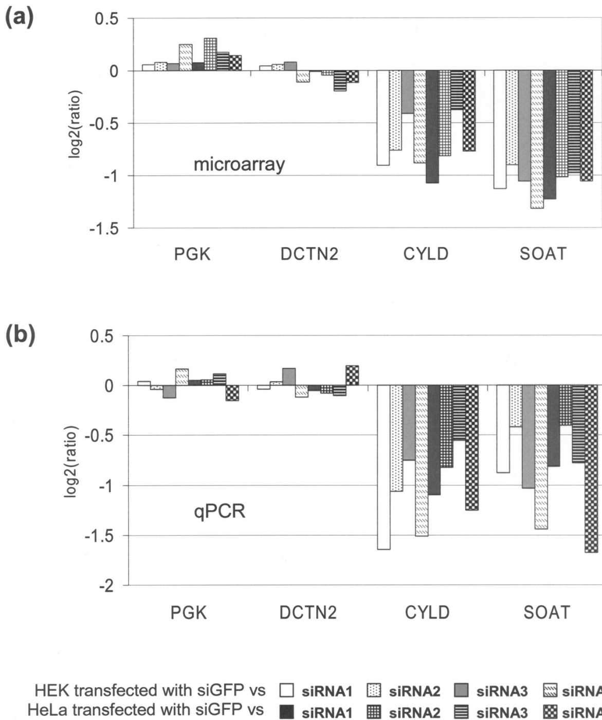
Figure 1 A siRNA directed against GFP specifically targets endogenous genes in human cells. (a) After transfection of the control siRNA directed against GFP , underrepresentation of the off-target genes CYLD and SOAT was detected by expression-microarrays 48 h post-transfection in HEK and HeLa cells. Normalization was performed as described in Additional file 5. (b) Verification of underrepresentation of CYLD and SOAT in HEK and HeLa cells by Real-Time PCR using the same mRNA as template. Expression of genes was normalized to the median of 2 housekeeping genes ( PGK , DCTN2 ).
